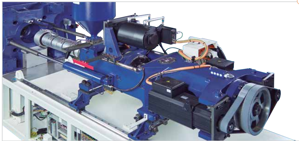
Image ① The new Zhafir Zeres Series - from 400 to 13,800 kN. With up to 4 injection units per clamping units available.
